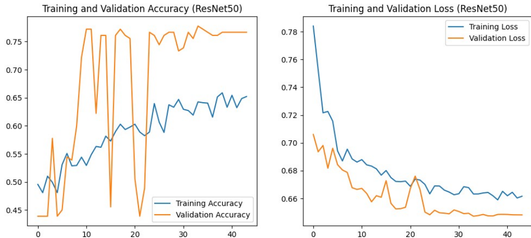
Gambar 4.3 Grafik Perbandingan Kurva Training dan Validation Accuracy & Loss Arsitektur ResNet50
