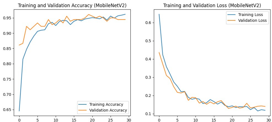
Gambar 4.4 Grafik Perbandingan Kurva Training dan Validation Accuracy & Loss Arsitektur MobileNetV2
