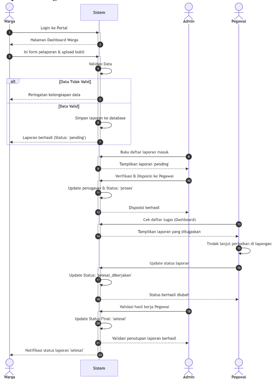
Gambar 4.5 Sequence Diagram
