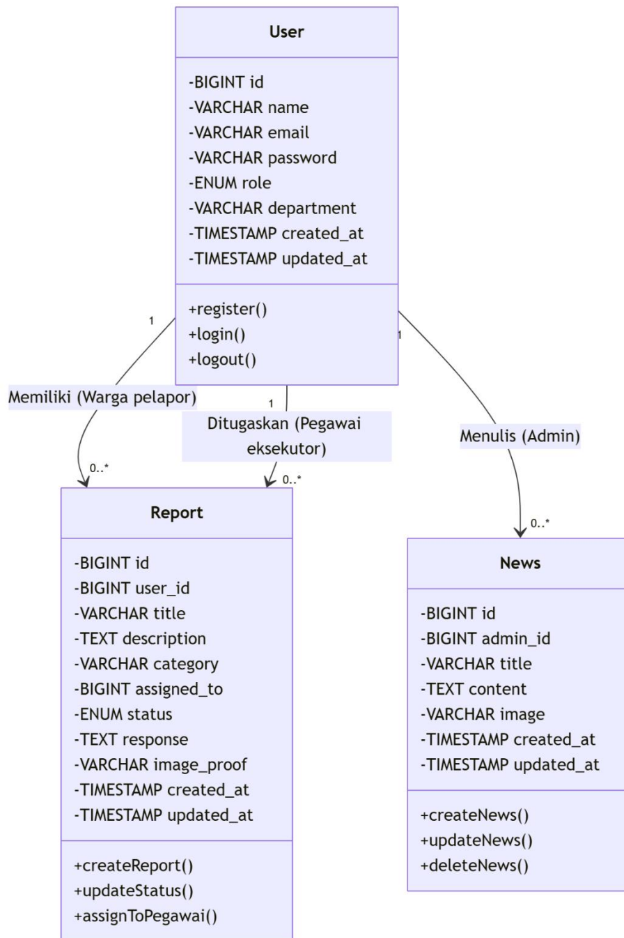
Gambar 4.4 Class Diagram
