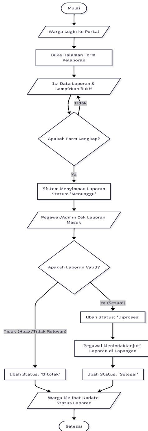
Gambar 4. 1 Flowchart
