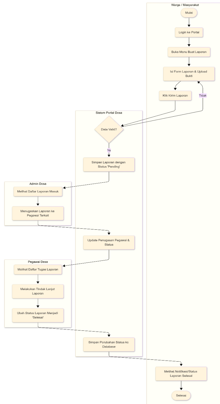
Gambar 4. 3 Activity Diagram
